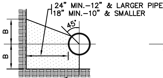
SECTION X-X BENDS & TEES
