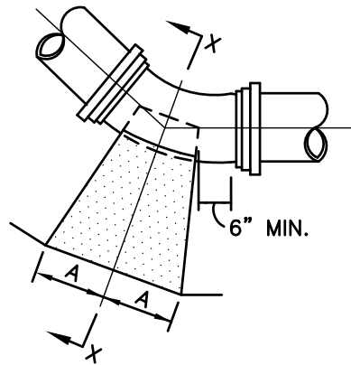
PLAN BENDS
