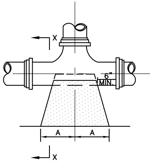
PLAN TEES
